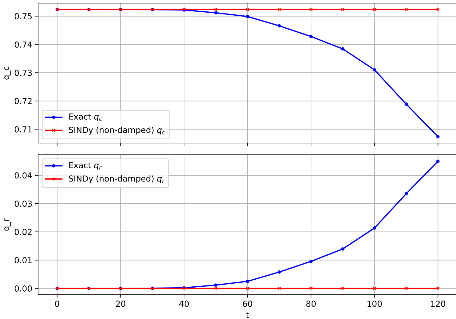
Trajectory 963 (non-damped)
