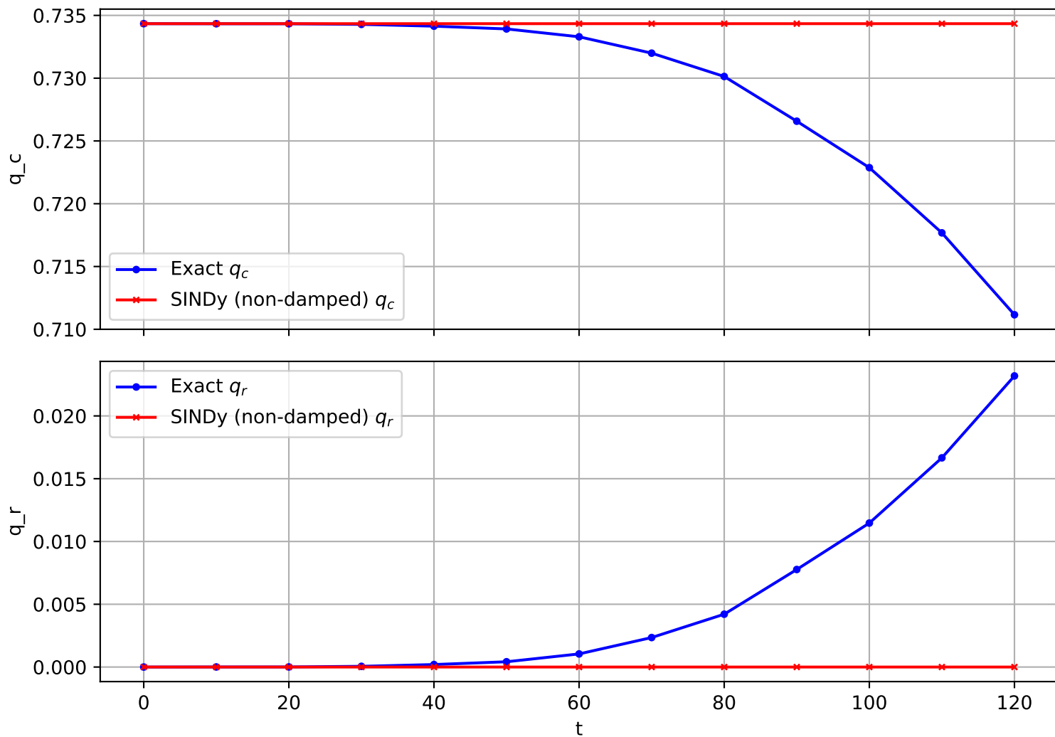
Trajectory 971 (non-damped)
