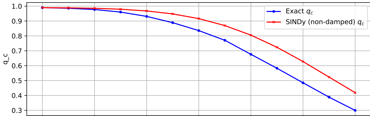
Trajectory 976 (non-damped)
