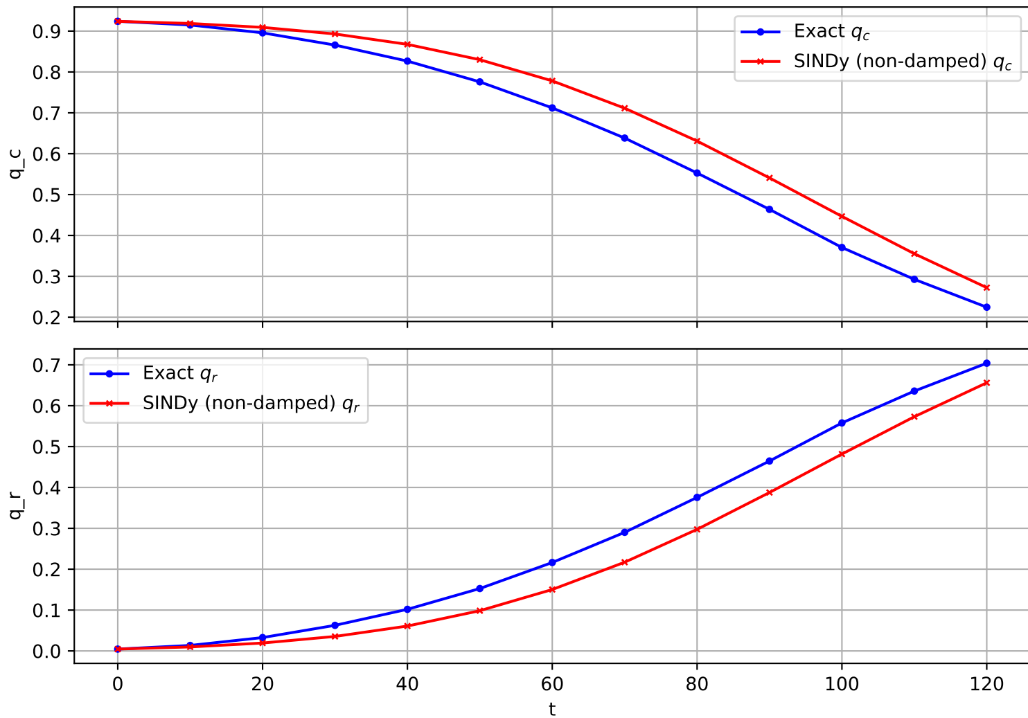
Trajectory 979 (non-damped)
