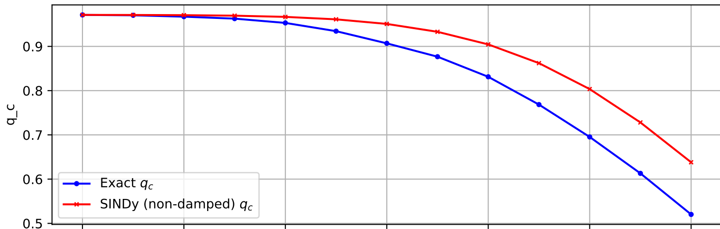
Trajectory 986 (non-damped)
