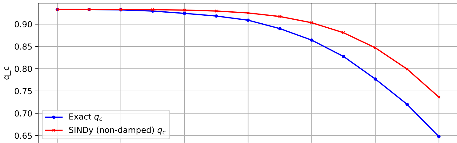
Trajectory 995 (non-damped)
