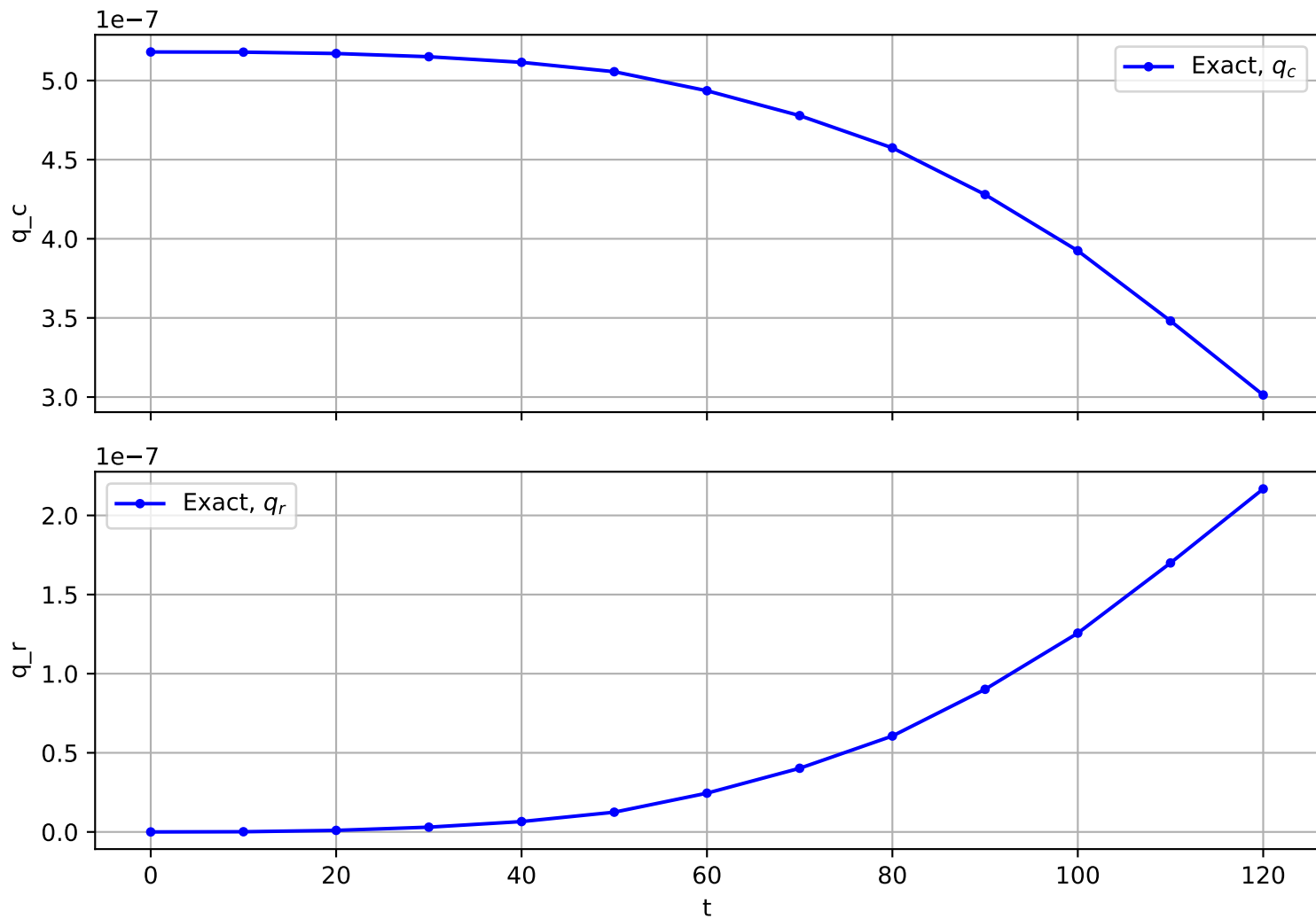
Trajectory No. 1002
