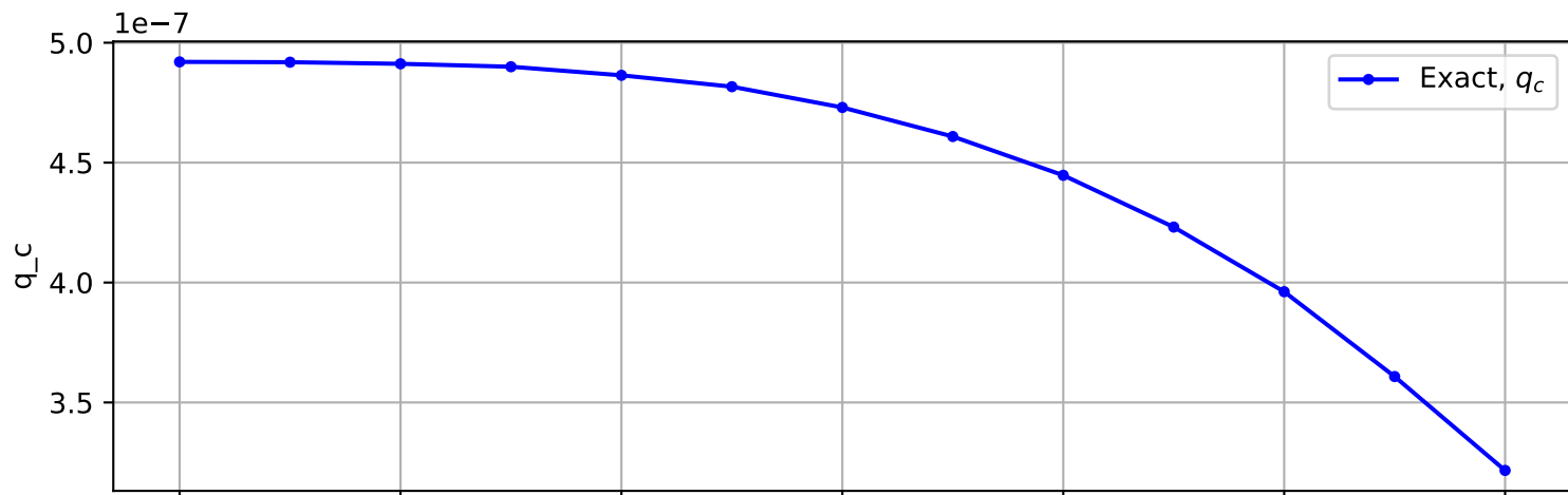
Trajectory No. 1003
