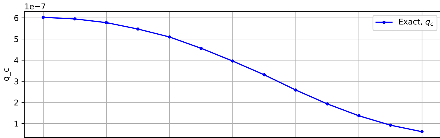
Trajectory No. 1012
