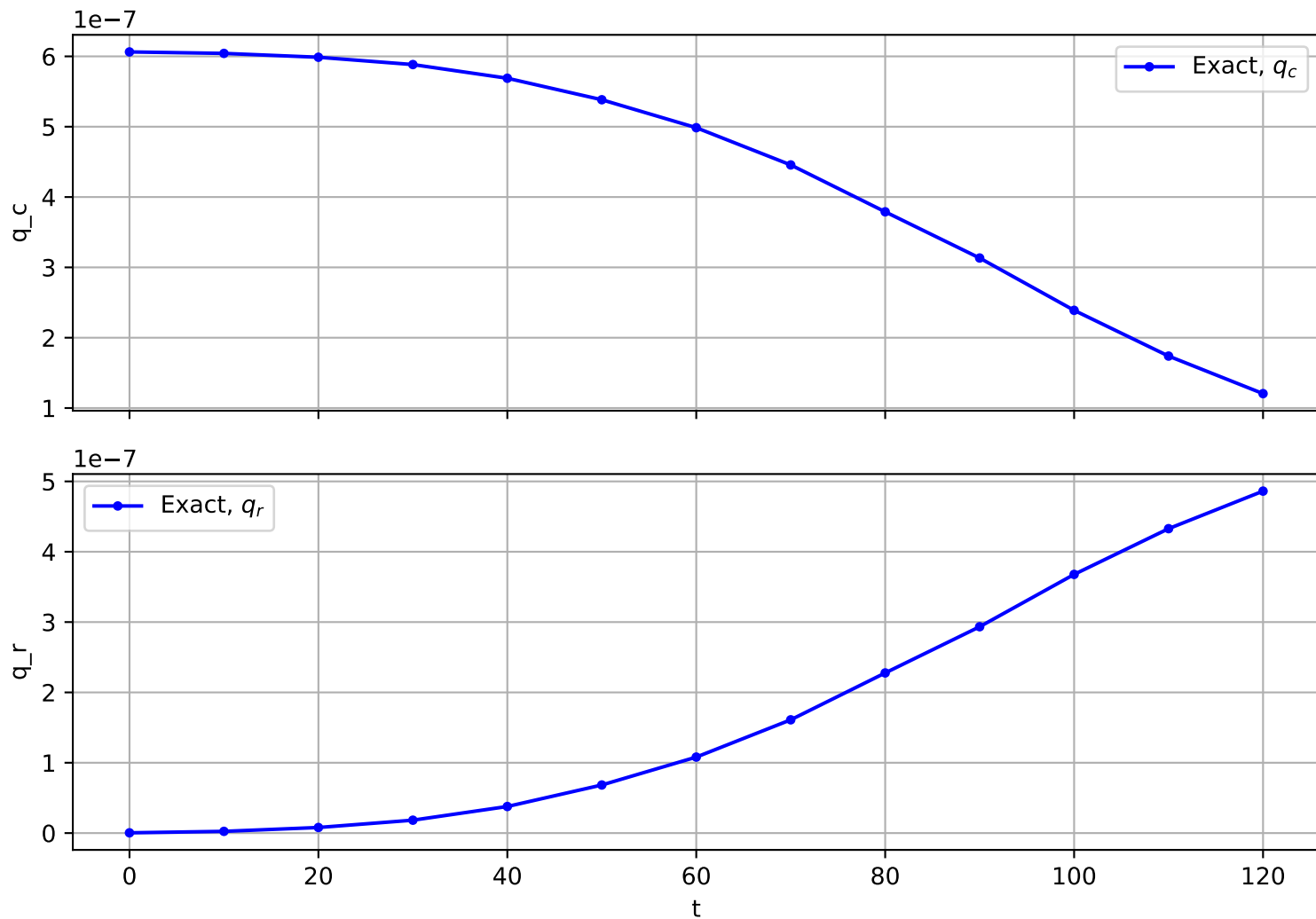
Trajectory No. 1019
