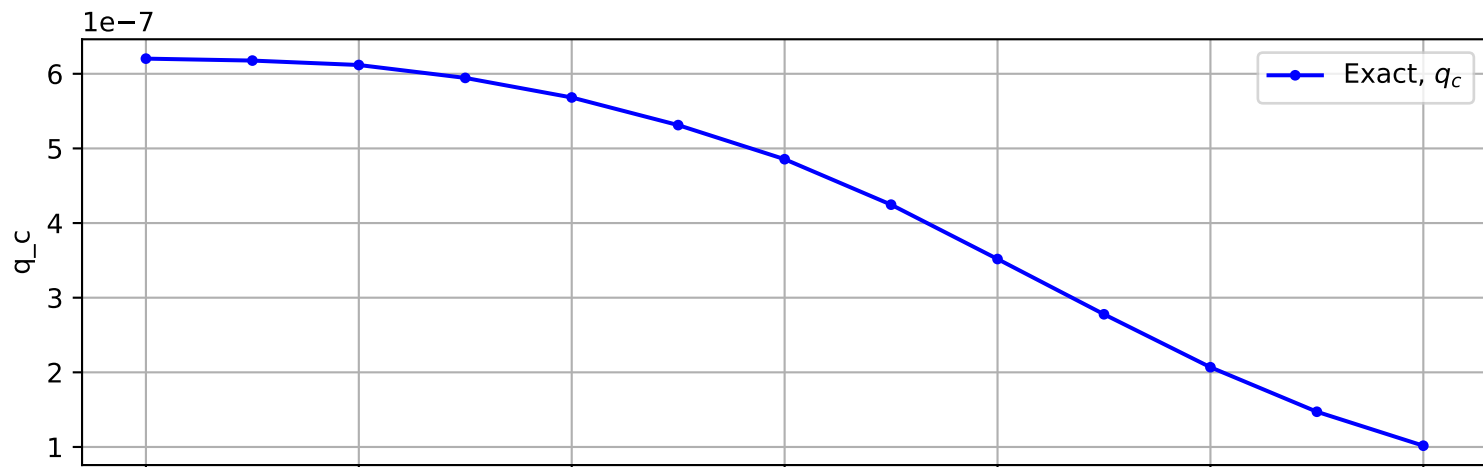
Trajectory No. 1022
