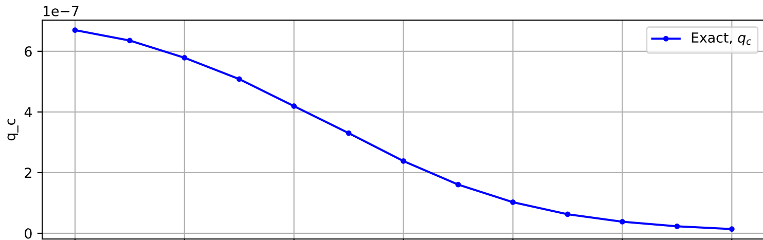
Trajectory No. 1053
