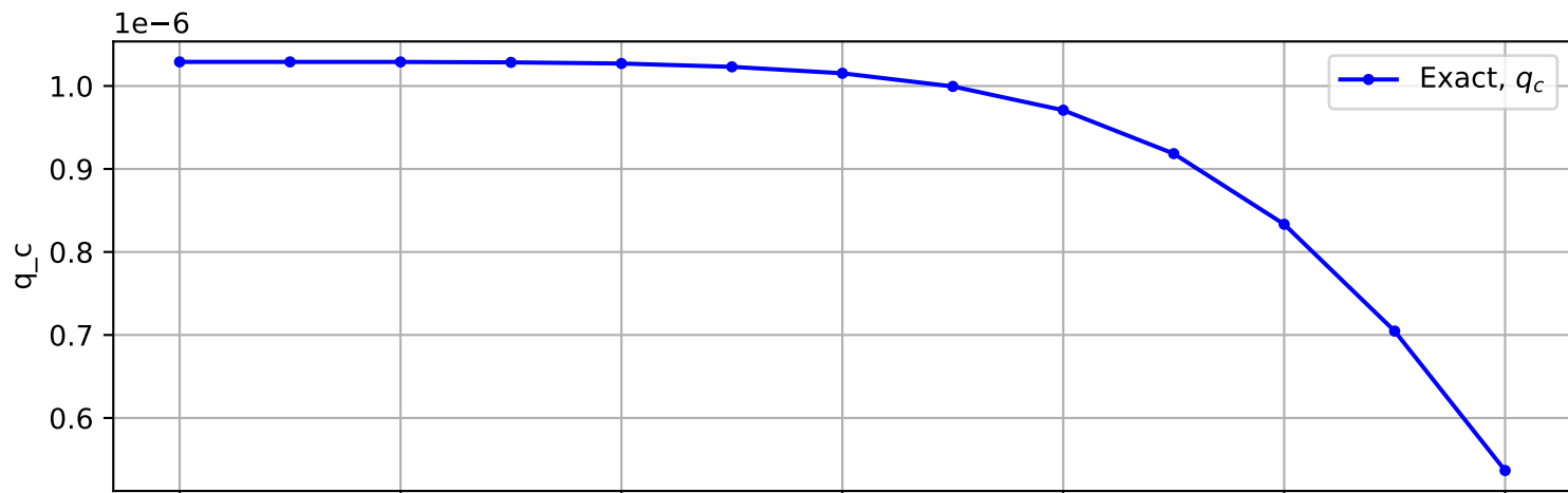
Trajectory No. 111
