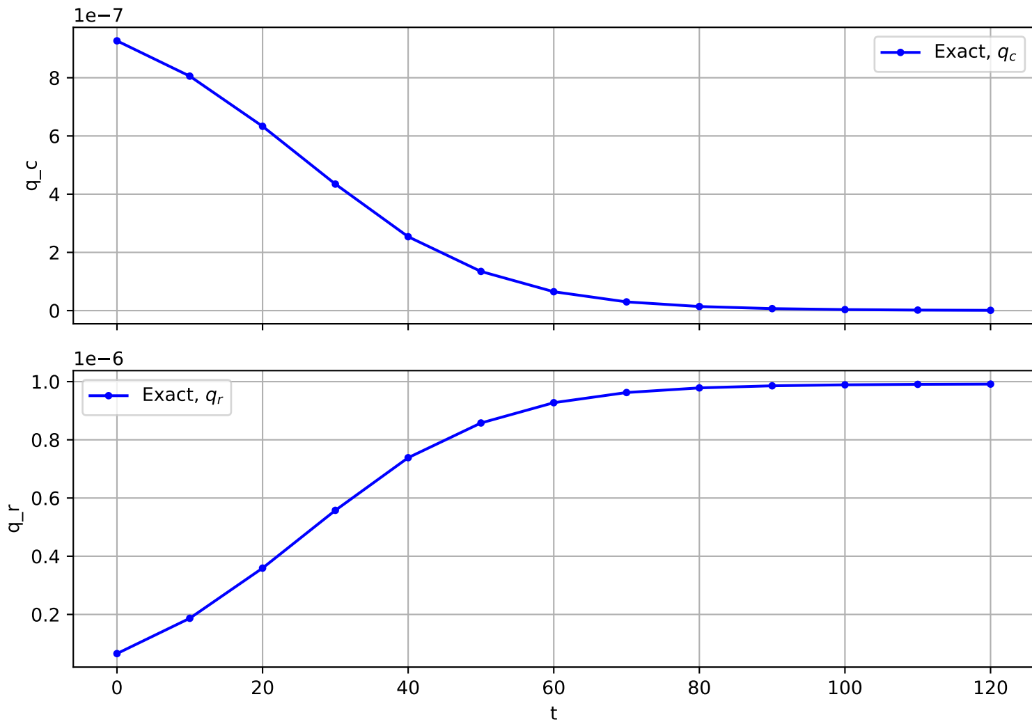
Trajectory No. 1152
