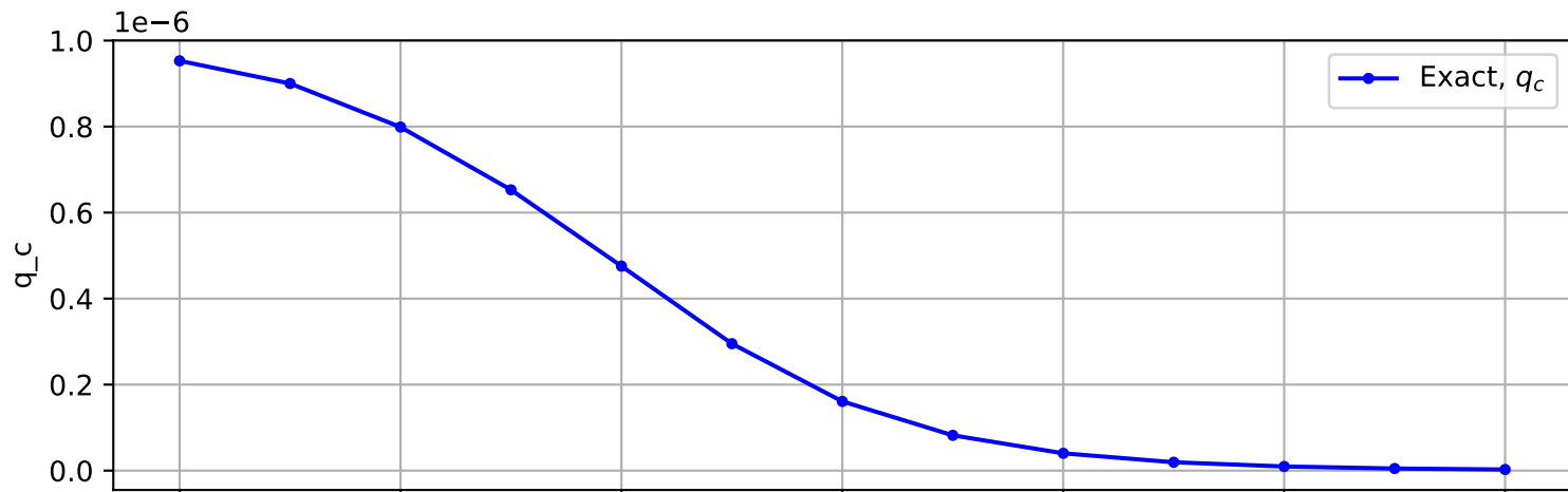
Trajectory No. 1175
