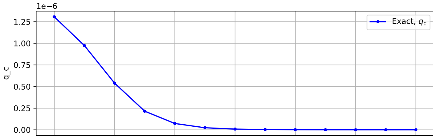
Trajectory No. 1242
