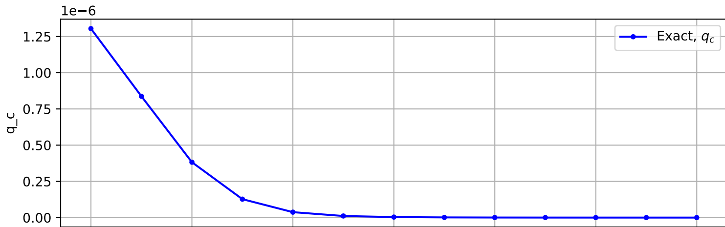
Trajectory No. 1283
