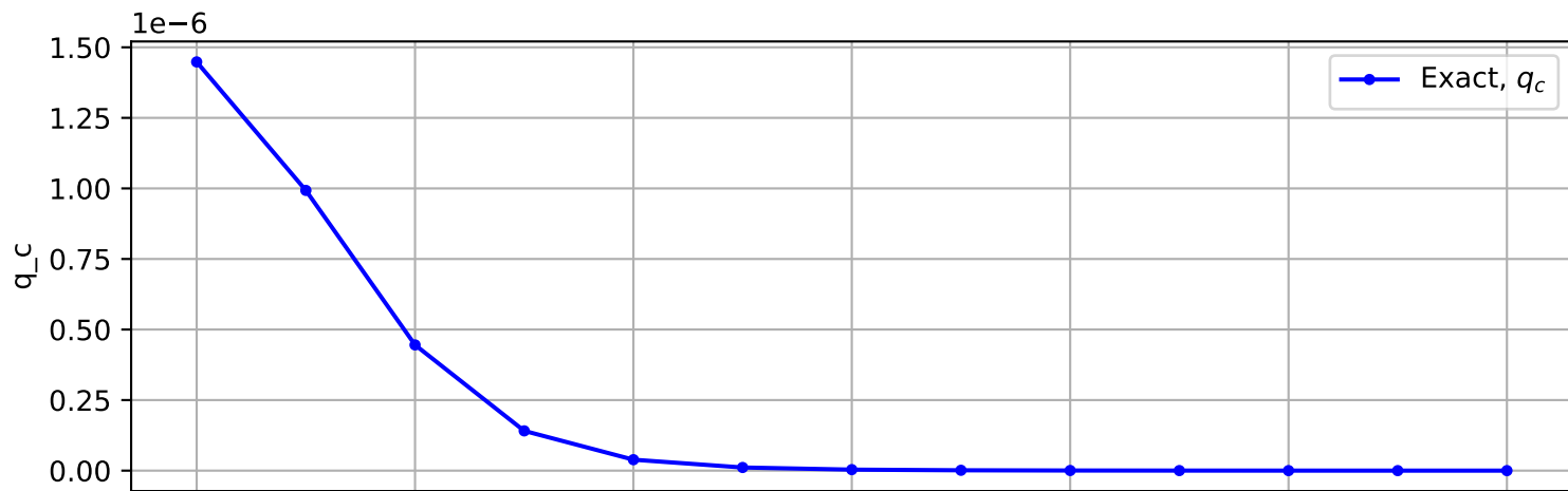
Trajectory No. 1285
