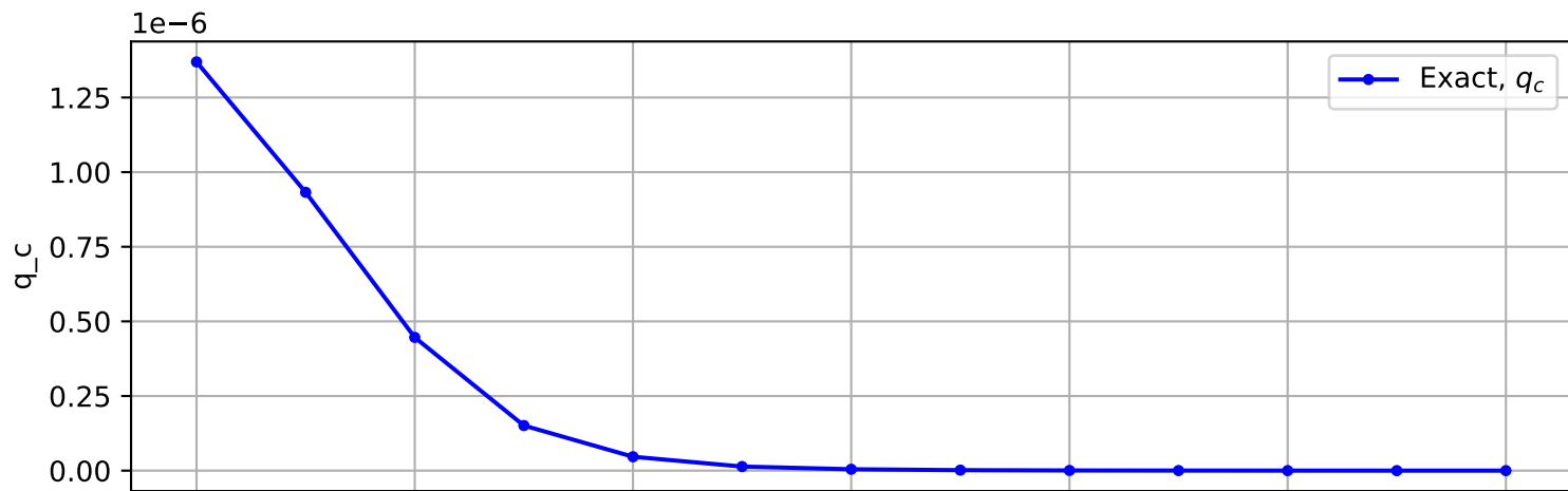
Trajectory No. 1288
