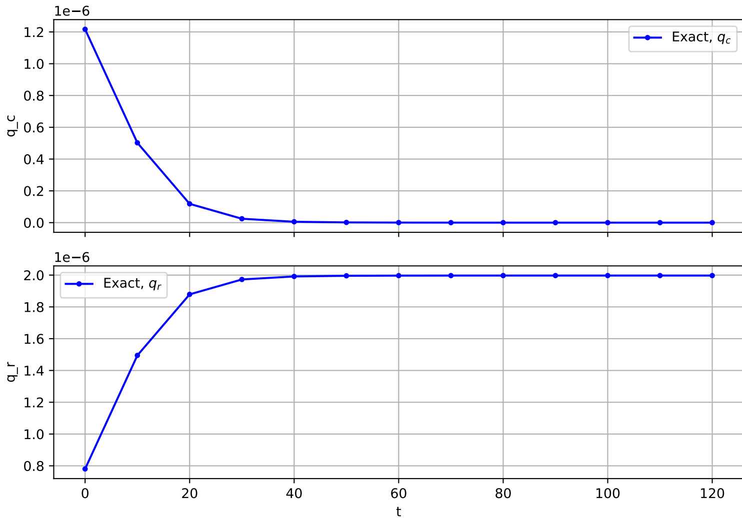
Trajectory No. 1299
