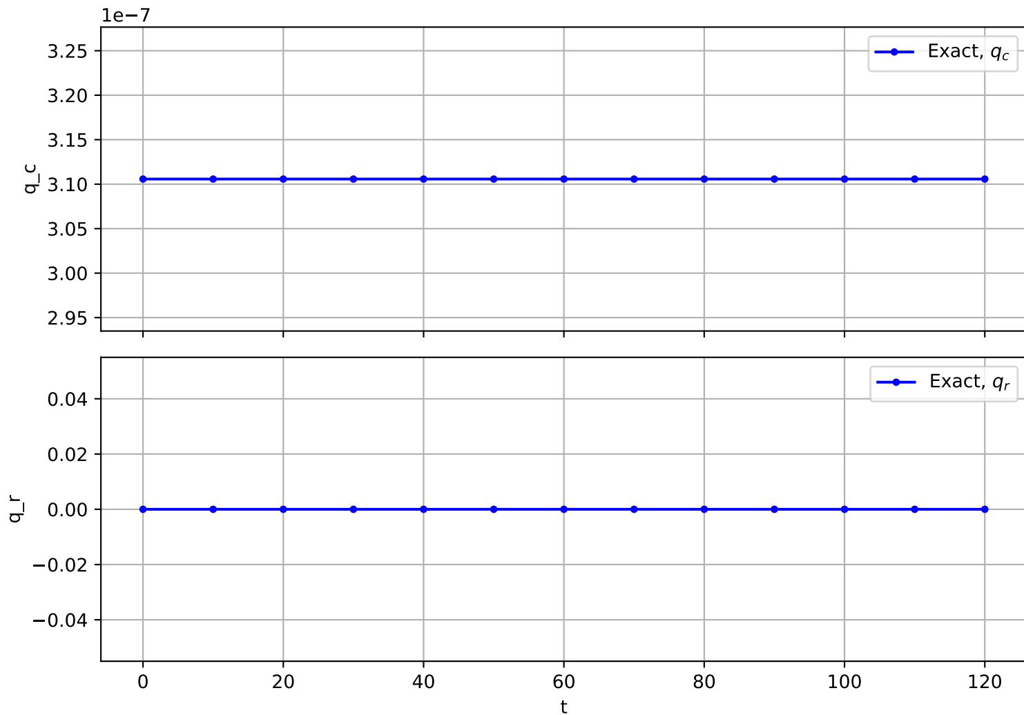
Trajectory No. 1337
