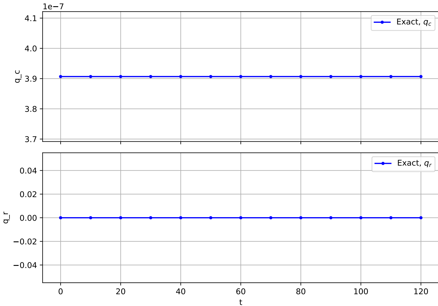
Trajectory No. 1338
