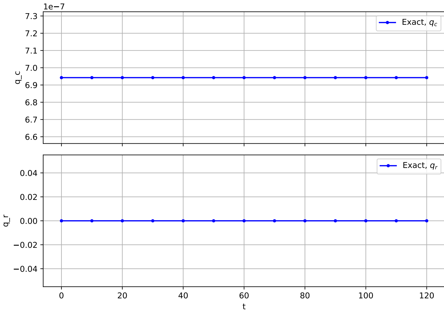
Trajectory No. 1359
