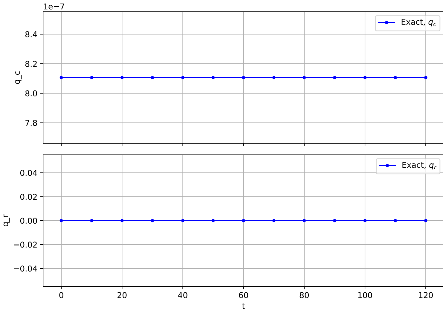
Trajectory No. 1368
