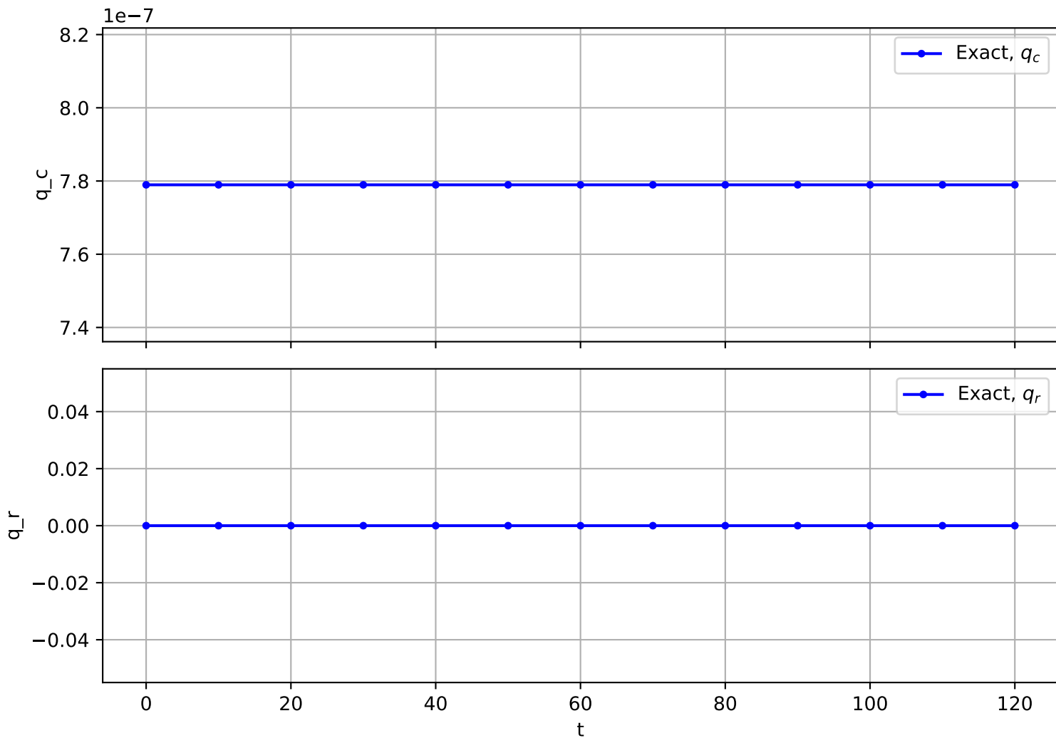
Trajectory No. 1371
