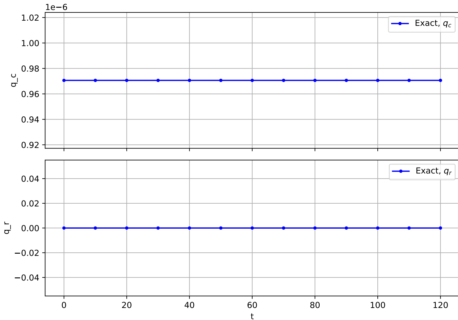
Trajectory No. 1382
