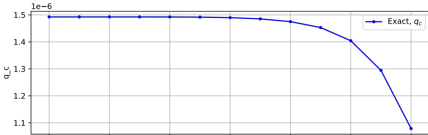
Trajectory No. 1398
