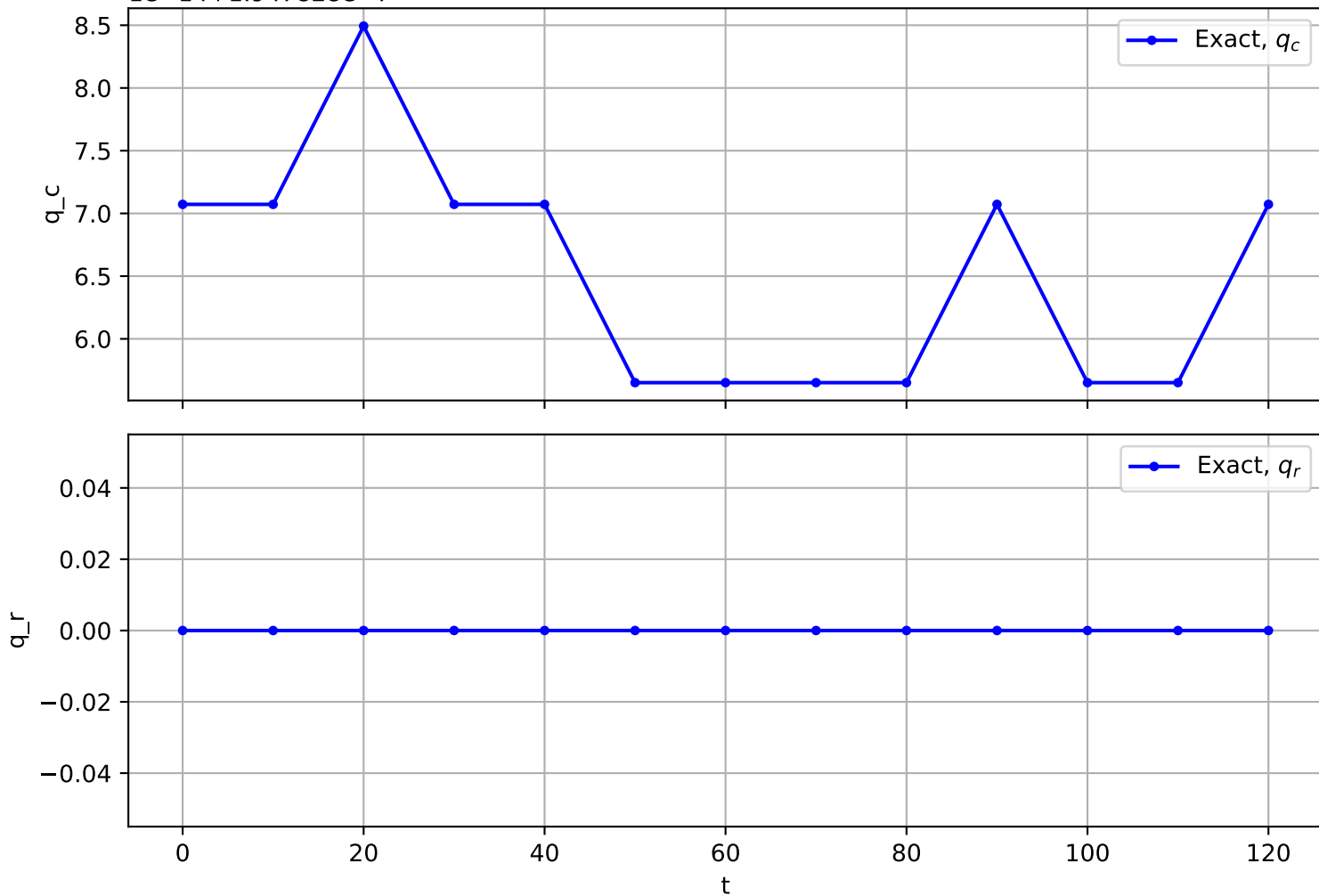
Trajectory No. 1445
