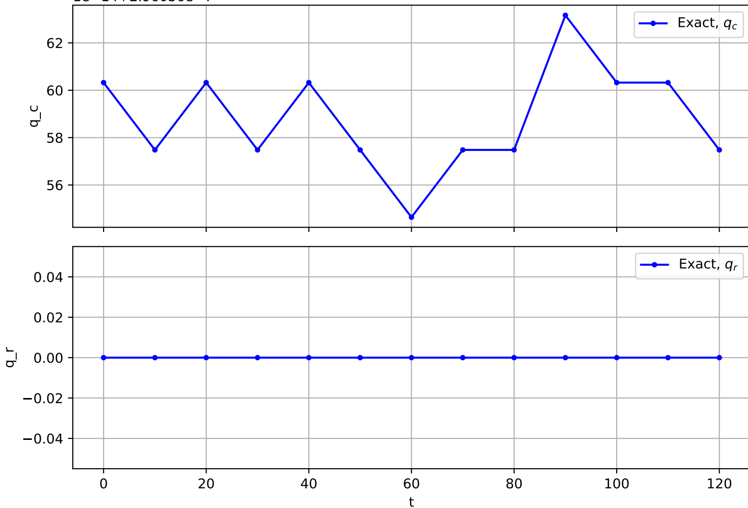
Trajectory No. 1457
