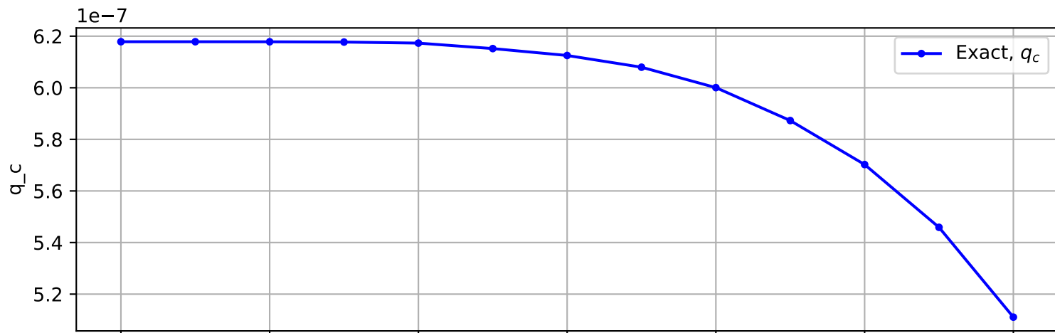
Trajectory No. 1511
