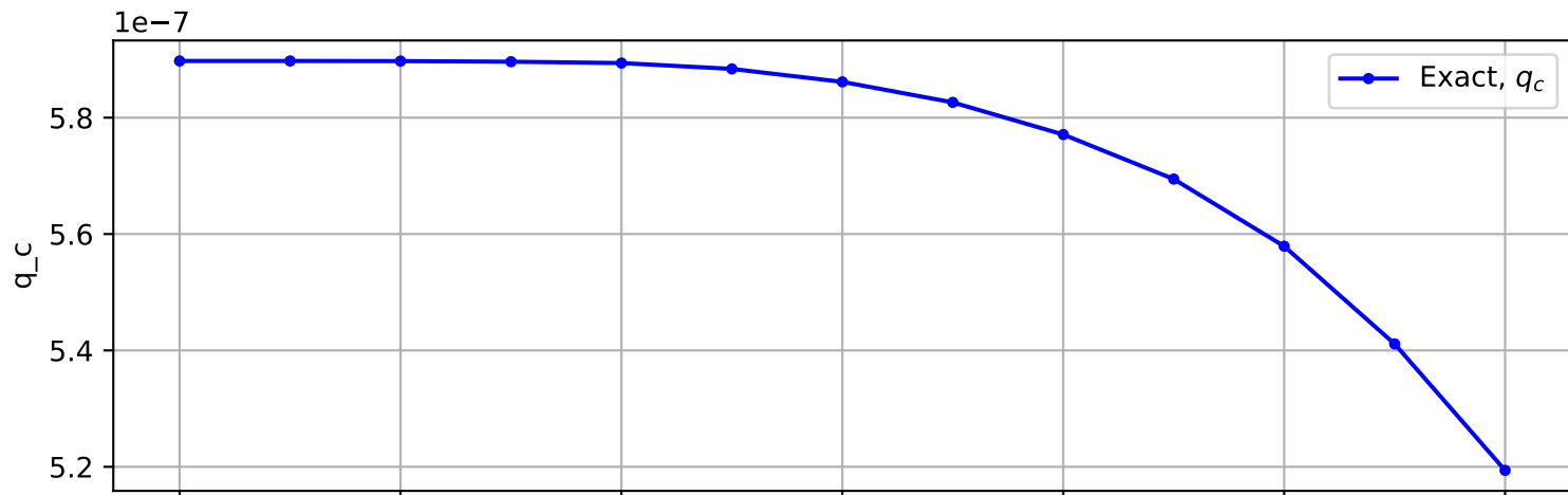
Trajectory No. 1512
