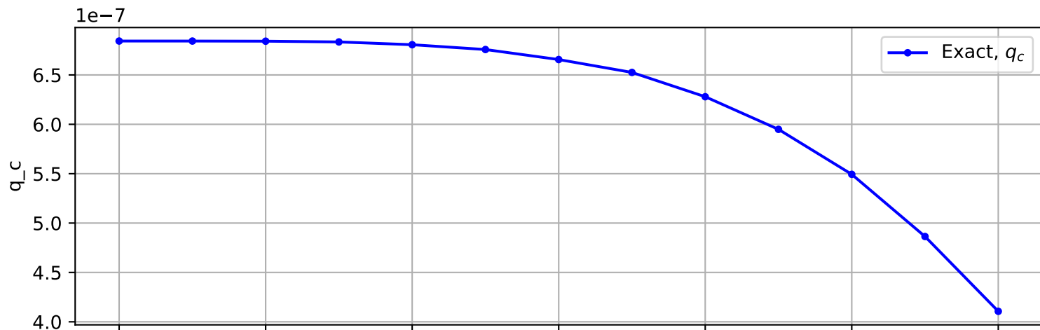
Trajectory No. 1544
