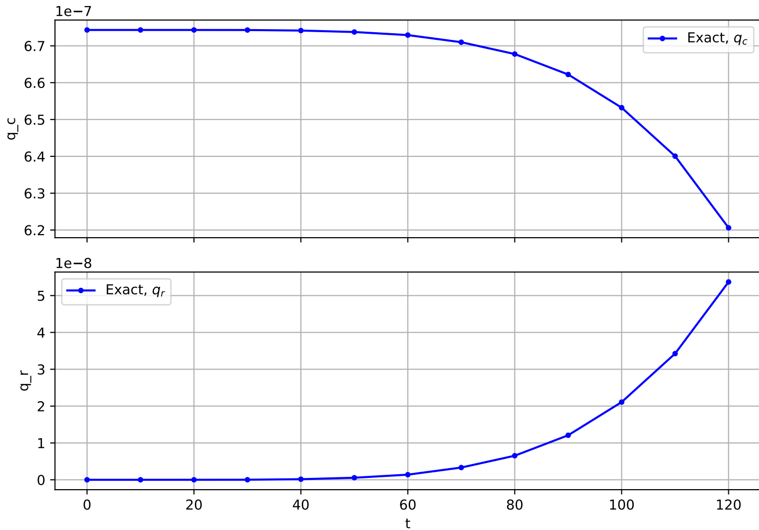
Trajectory No. 1558
