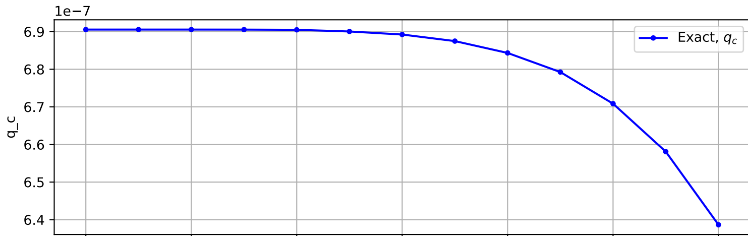
Trajectory No. 1559
