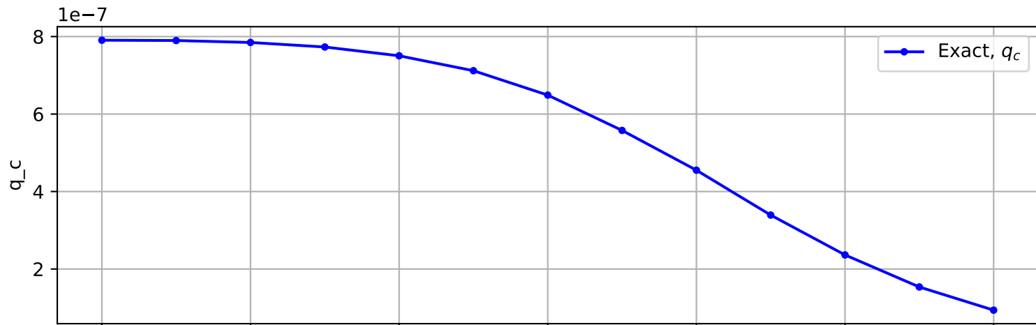
Trajectory No. 1560
