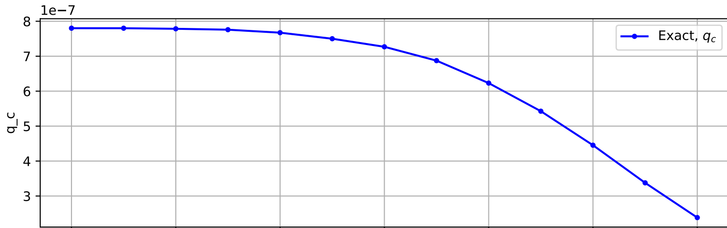
Trajectory No. 1573
