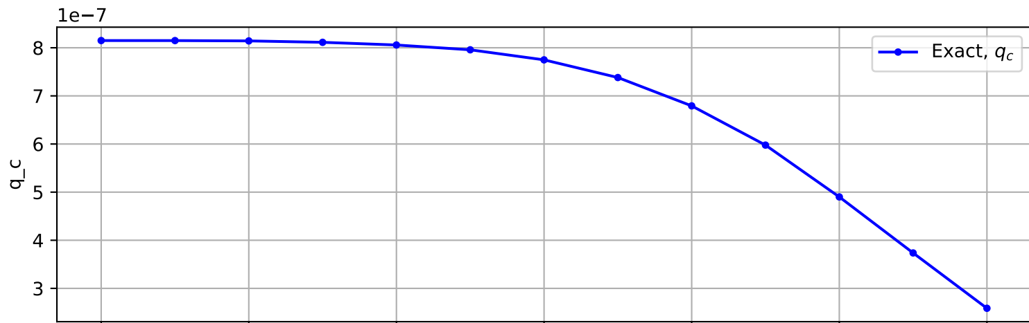
Trajectory No. 1574
