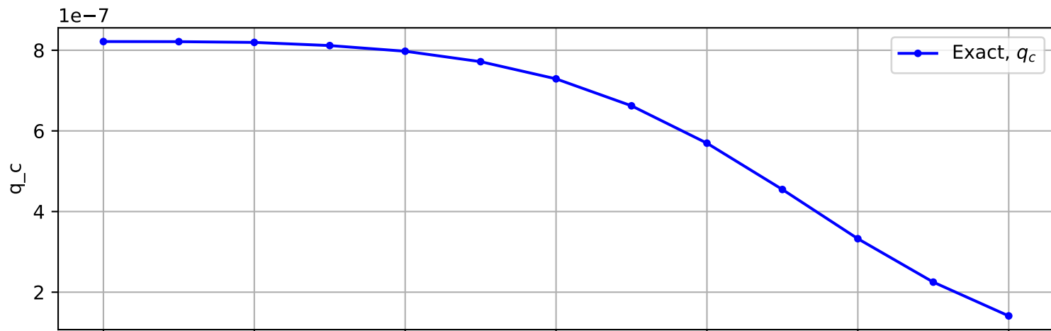
Trajectory No. 1577
