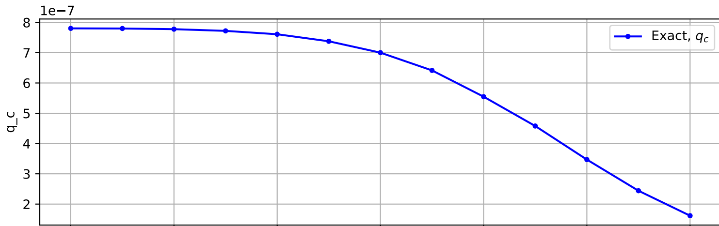
Trajectory No. 1578
