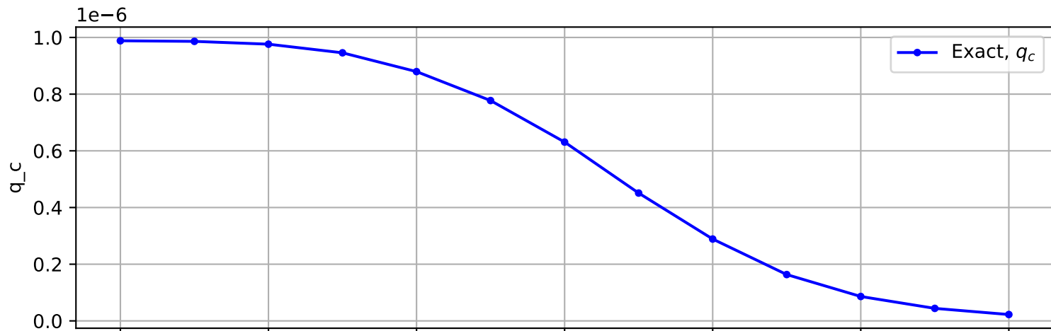
Trajectory No. 1646
