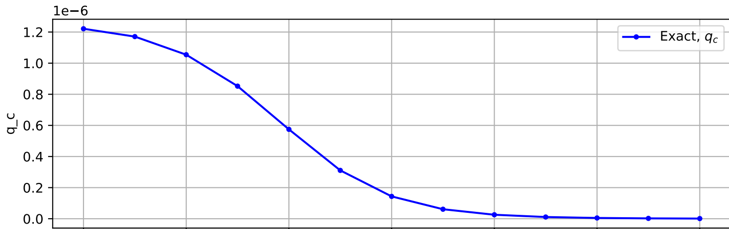
Trajectory No. 1670
