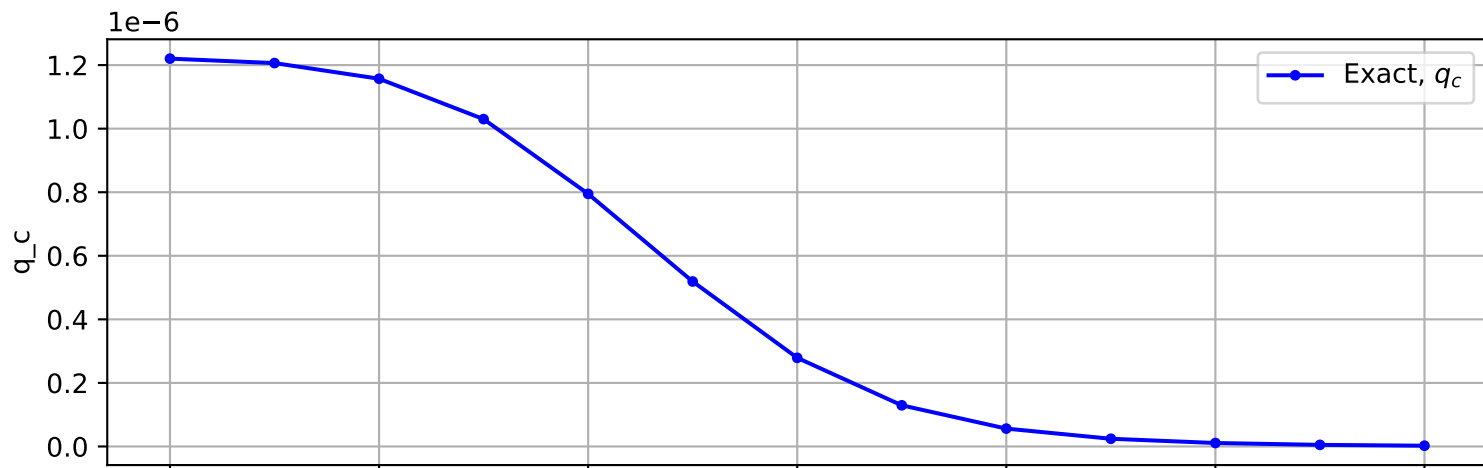
Trajectory No. 1684
