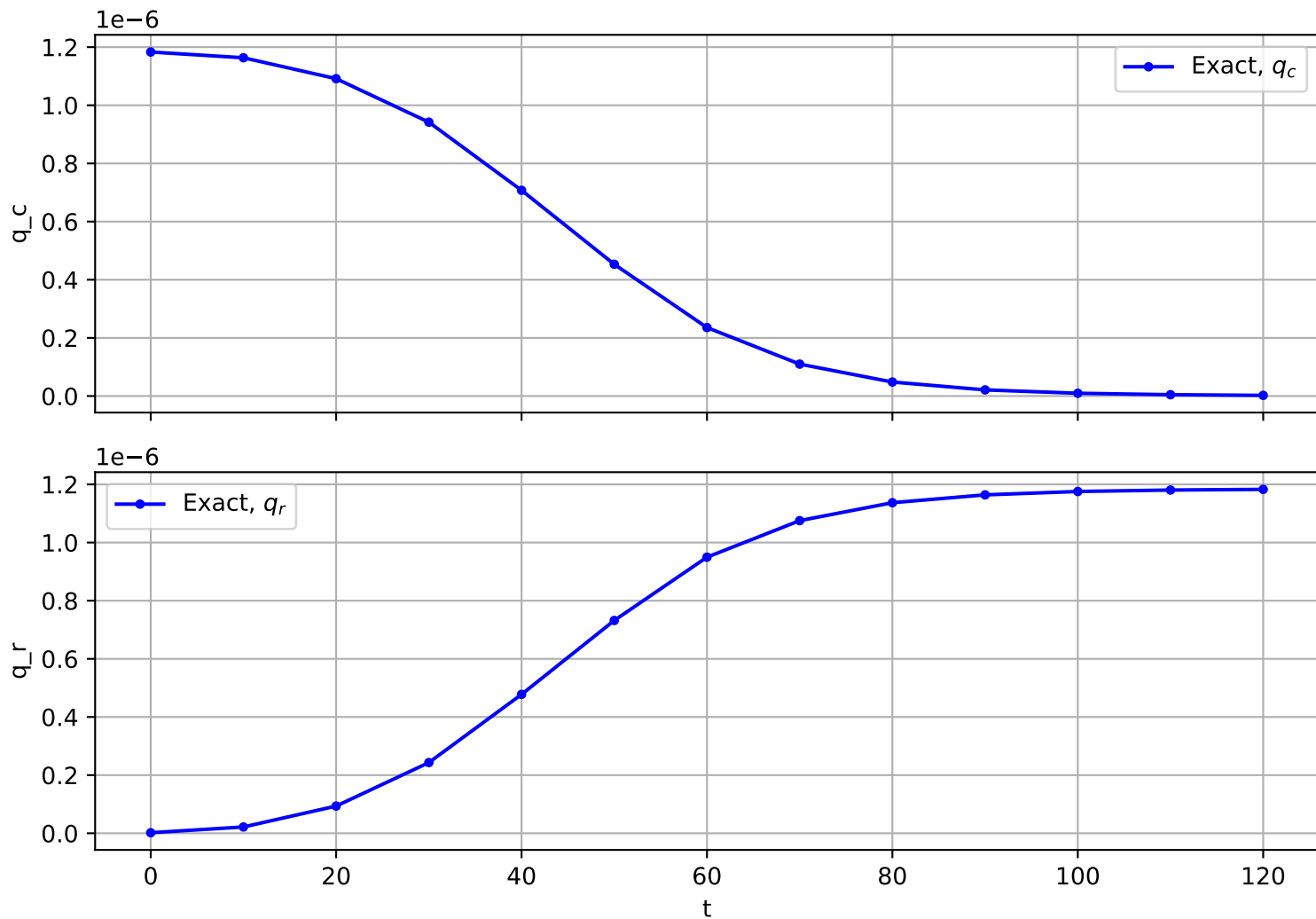
Trajectory No. 1687
