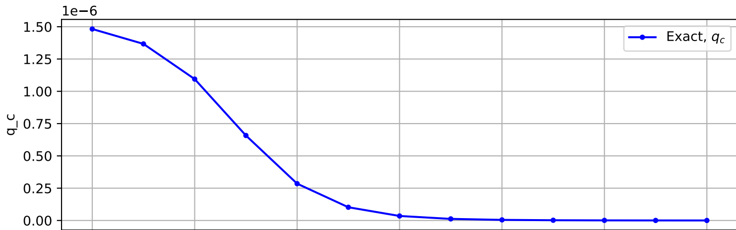
Trajectory No. 1723
