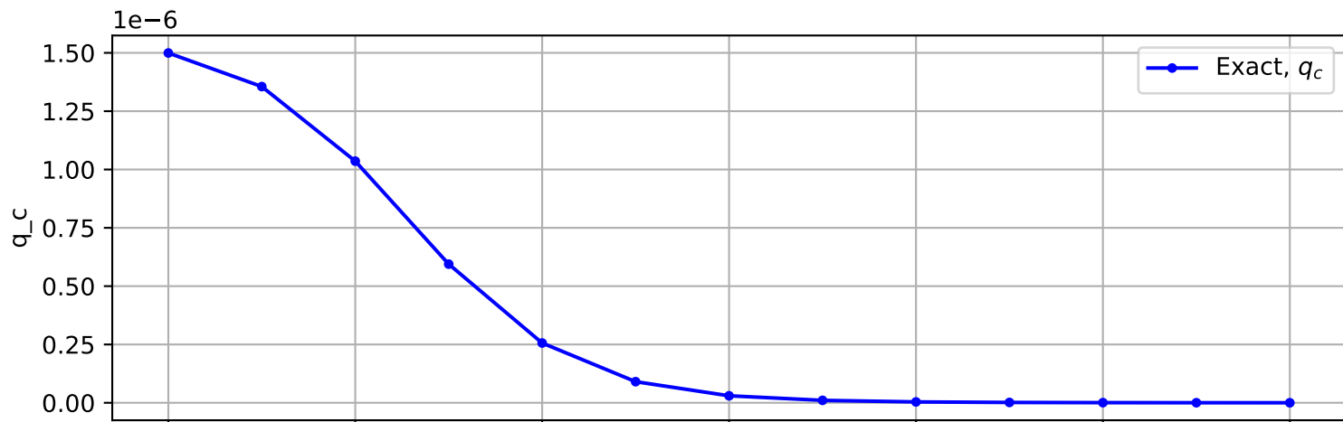
Trajectory No. 1724
