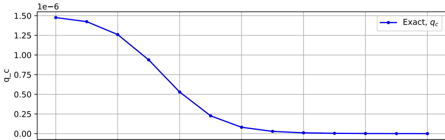
Trajectory No. 1725
