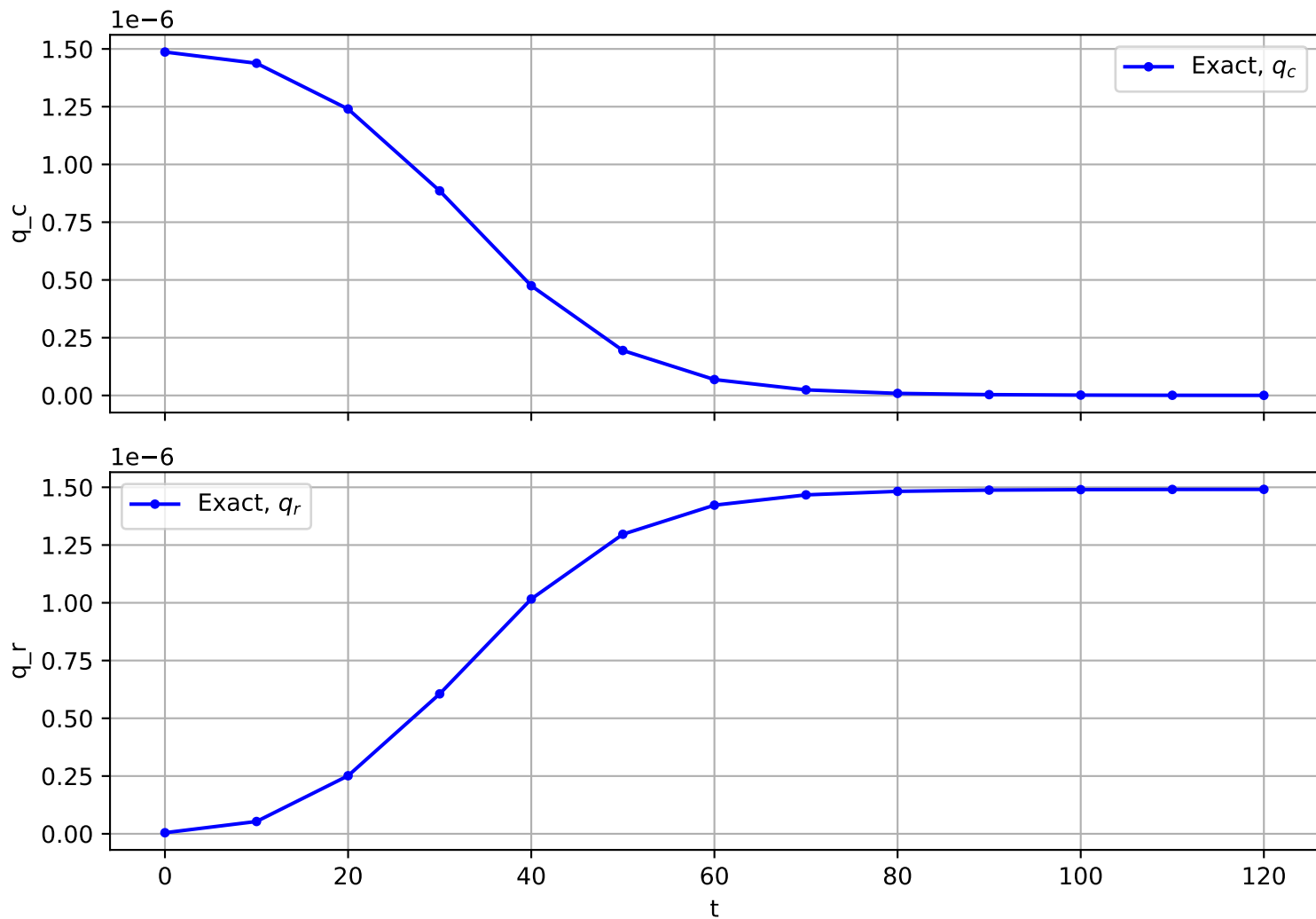
Trajectory No. 1729
