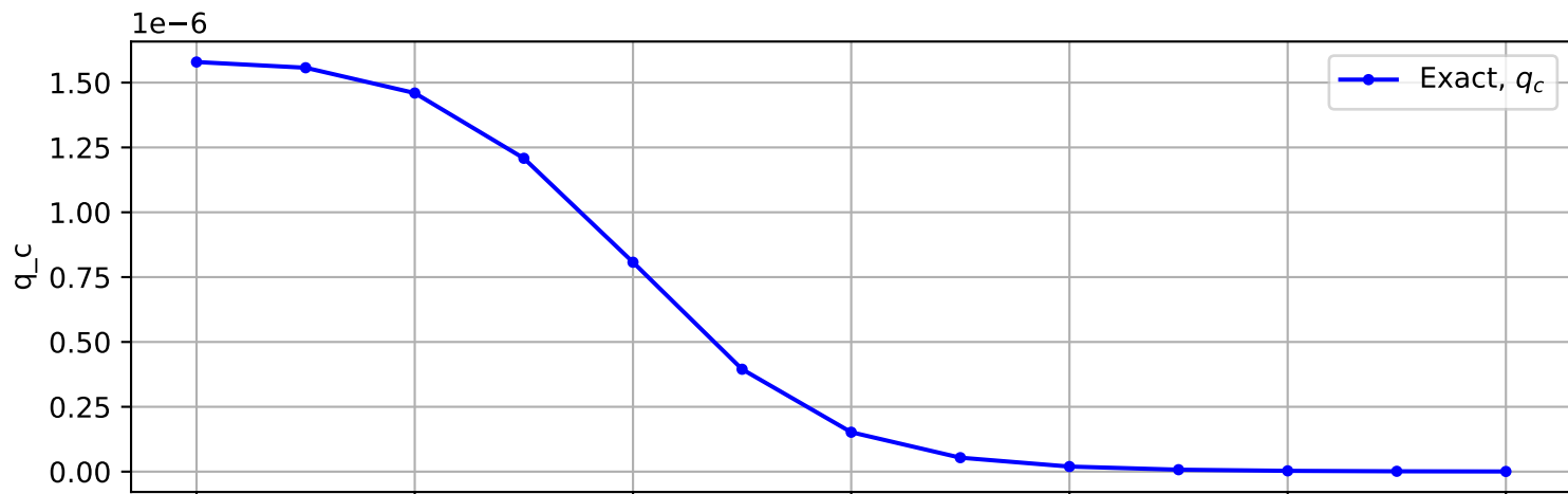
Trajectory No. 173
