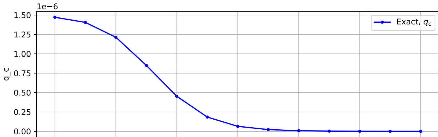
Trajectory No. 1730
