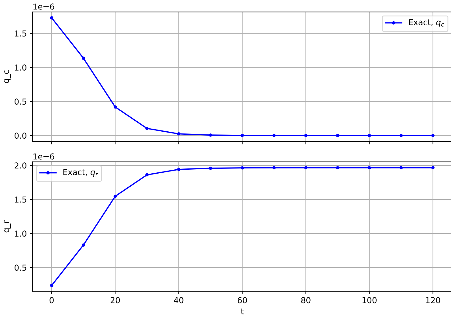
Trajectory No. 1777
